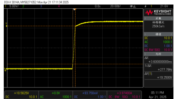
INPUT=230VAC/50HZ @ FULL LOAD CH1 : Output Voltage
